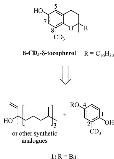
Figure 1. Retrosynthesis of ring-labeled \delta -tocopherol
