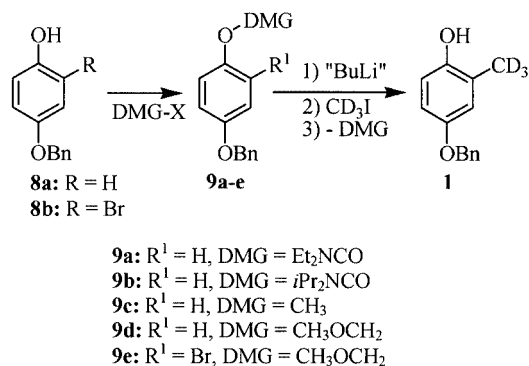
Scheme 2. Preparation of 1 by directed metallation (DMG = directing metallation group)
