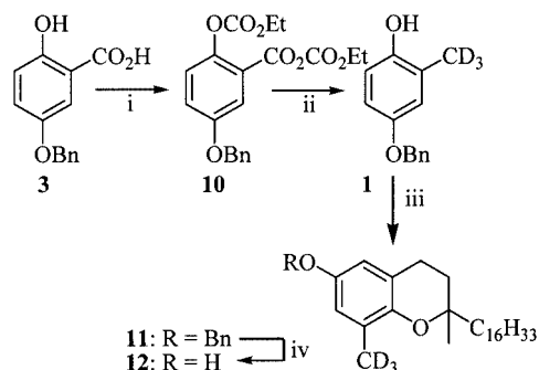
Scheme 3. i) \text{ClCO}_2\text{Et} , \text{Et}_3\text{N} , 0 °C, 2 h; ii) \text{NaBD}_4 , 8 equiv., \text{D}_2\text{O}/\text{THF} , 0 °C, 3 h, 89%; iii) \text{ZnCl}_2 , 1.5 equiv., t\text{BuOAc} , aq. \text{HCl}_{\text{cat}} , isophytol, 72%; iv) 5% \text{Pd/C} , \text{H}_2 , \text{EtOAc} , overnight, quant.
