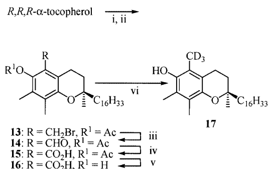
Scheme 4. i) \text{Br}_2 , hexane, room temp., 3 h; ii) \text{Ac}_2\text{O} , \text{AcOH} , \text{CH}_2\text{Cl}_2 , \text{H}_2\text{SO}_4 cat., room temp., overnight, 82% over 2 steps; iii) \text{NMO} , 4 equiv., \text{CH}_3\text{CN} , room temp., overnight, 92%; iv) \text{NH}_2\text{SO}_3\text{H} , \text{NaClO}_2 , 1,4-dioxane/ \text{H}_2\text{O} , room temp., 50 min, 96%; v) \text{KOH} 2 M, \text{MeOH} , 50 °C, 2 h, 93%; vi) a. \text{ClCO}_2\text{Et} , \text{Et}_3\text{N} , 0 °C, 2 h, quant. b. \text{NaBD}_4 , 8 equiv., \text{D}_2\text{O}/\text{THF} , 0 °C, 3 h, 72%
